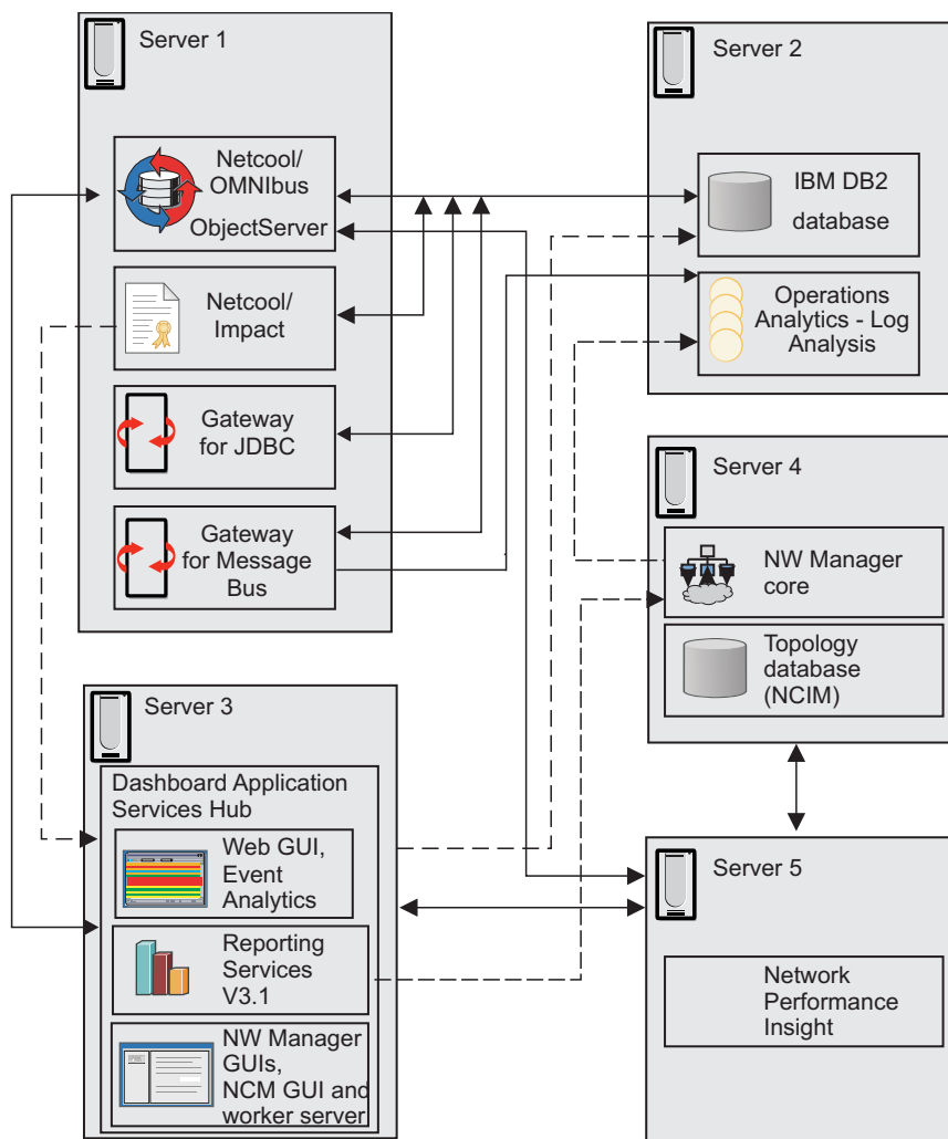
Figure 7. Simplified installation architecture for the installation scenario
